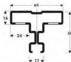
UPRIGHT SECTION SERIES USR
