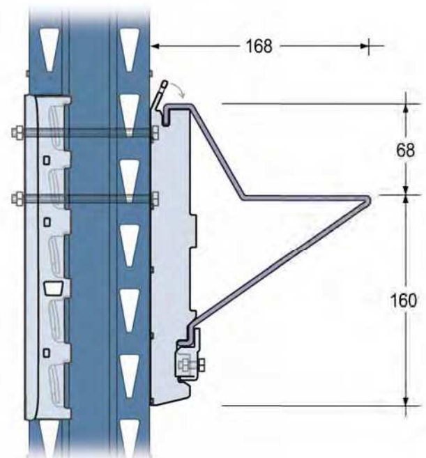
22 Double sided DRIVE-IN guide rails located on single brackets
